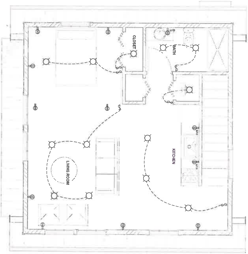
FIRST FLOOR ELECTRICAL PLAN SCALE: 1/2" = 1'
